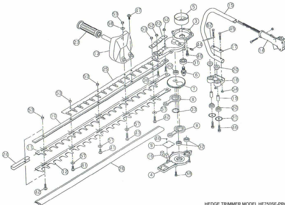
HEDGE TRIMMER MODEL HF750SF-PRO
